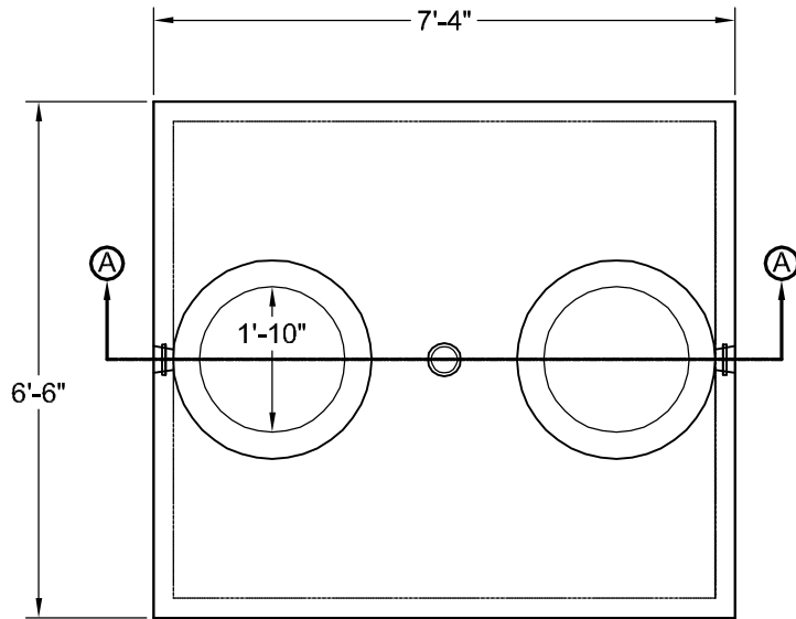
PLAN VIEW
